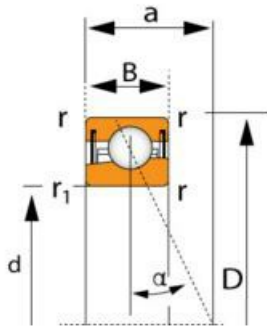
B71900-2RZ Ultra high-speed Sealed angular contact ball bearings (ISO19)
